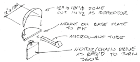
1/2" ISOMETRIC - DIRECTIONAL ANTENNA
